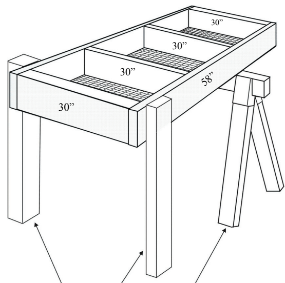
Figure 3. 4 x 4 legs or 2 x 4 legs or sawhorse support options shown in perspective view
